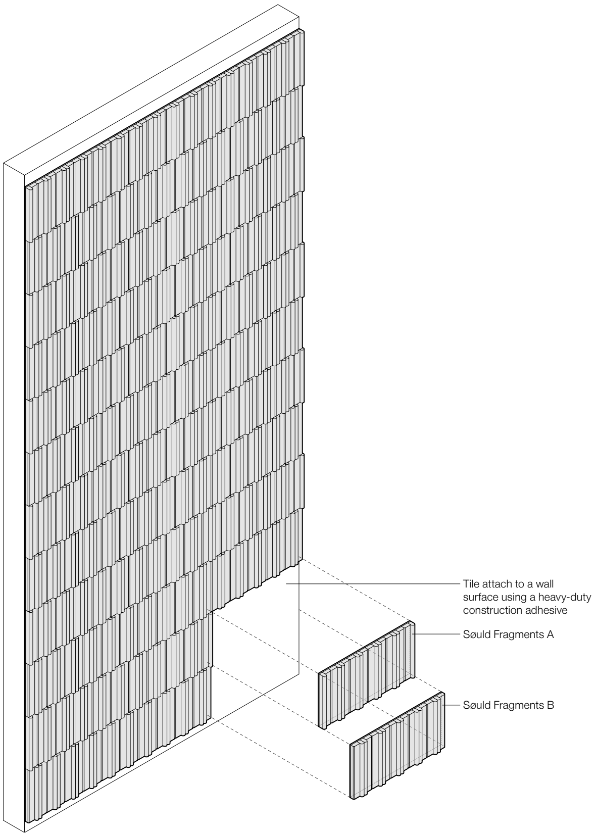
Exploded Axonometric Pattern 1 Shown
