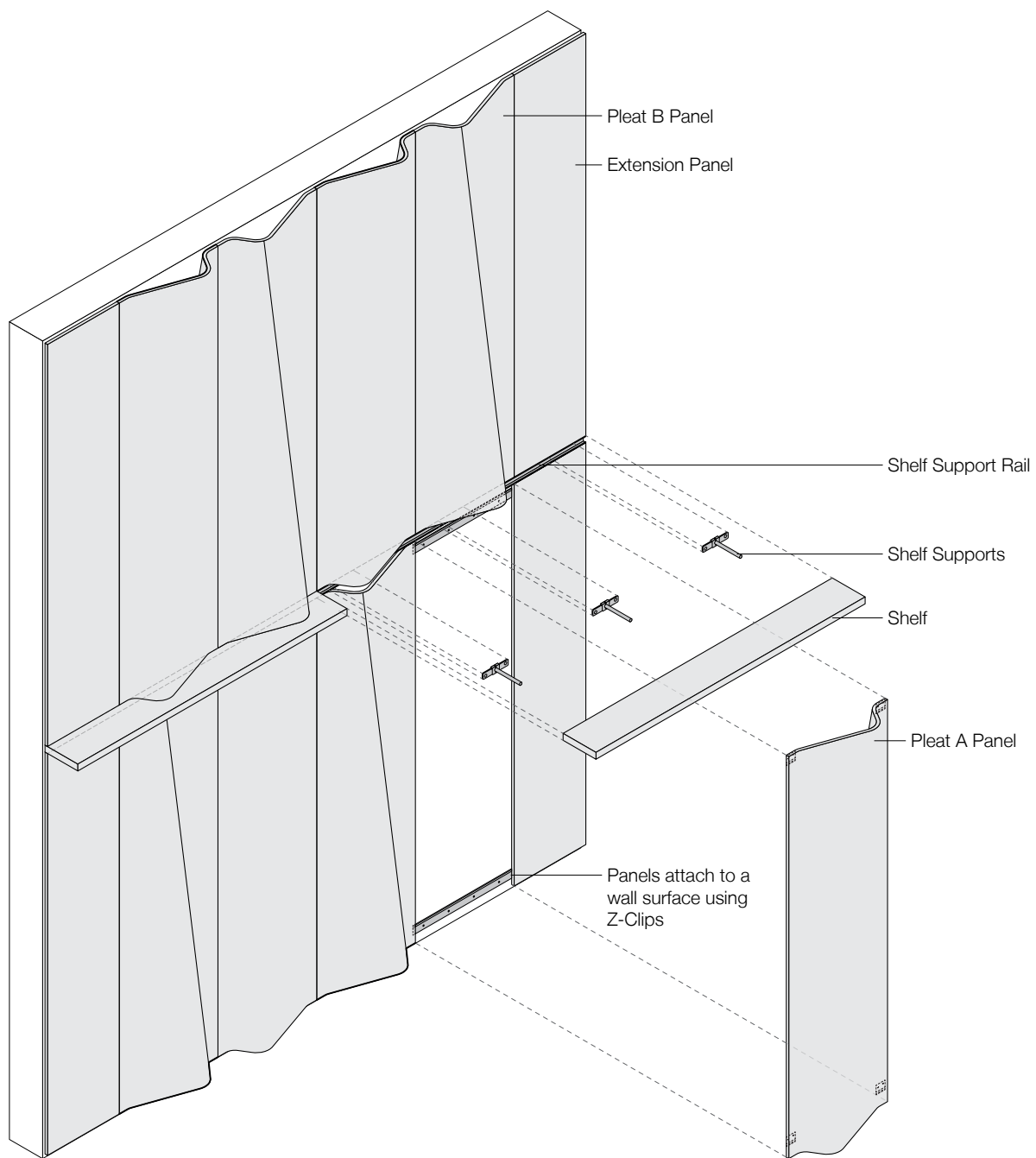
Exploded Axonometric
