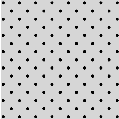
Pattern 457 Perforation Diameter: 0.052 in (1.32 mm) Density: 25 holes / in 2 (5 hole / cm 2 )
