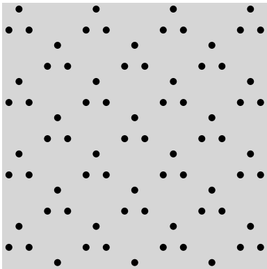
Pattern Multiple Diamond Perforation Diameter: 0.052 in (1.32 mm) Density: 22 holes / in 2 (4 hole / cm 2 )
