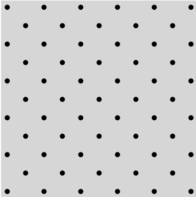
Pattern 330 Perforation Diameter: 0.052 in (1.32 mm) Density: 12 holes / in 2 (2 hole / cm 2 )
