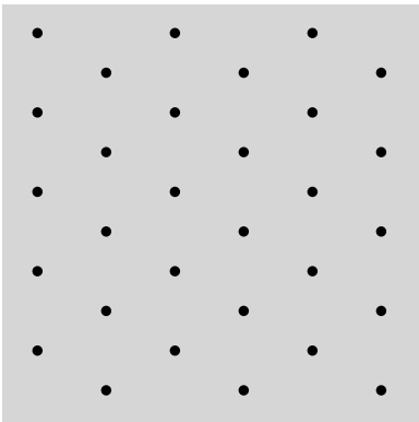
Pattern Euro MK 153 Perforation Diameter: 0.047 in (1.2 mm) Density: 12 holes / in 2 (3 hole / cm 2 )
