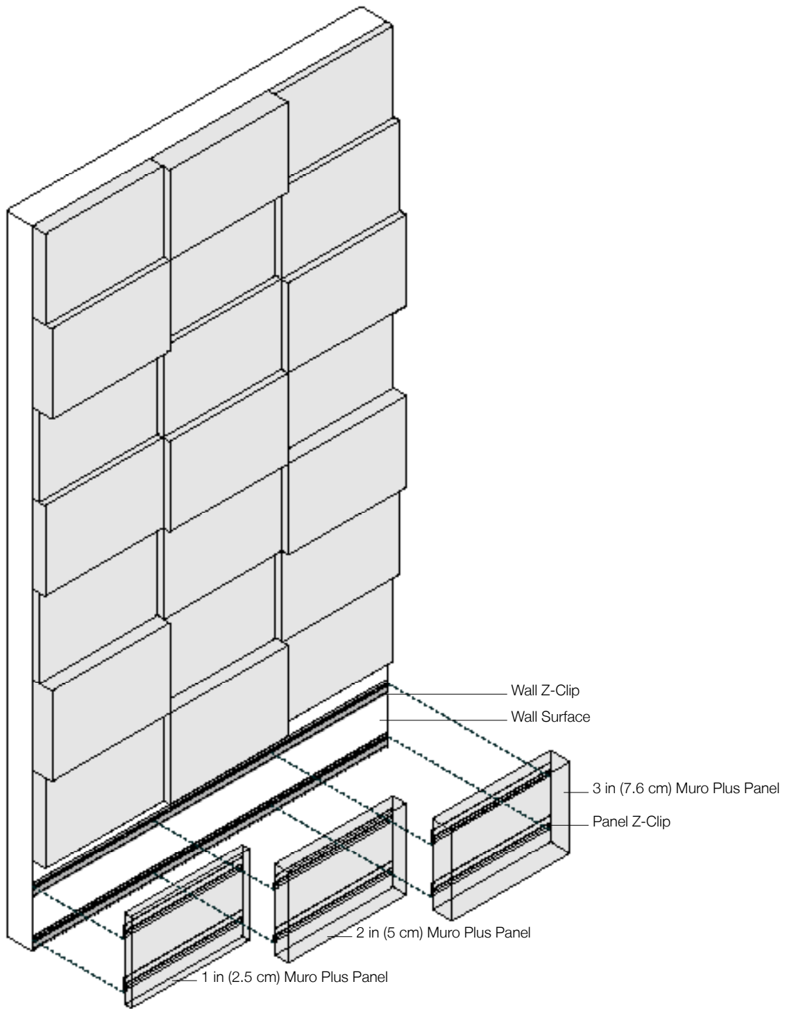
Exploded Axonometric Three Distinct Panel Thicknesses
