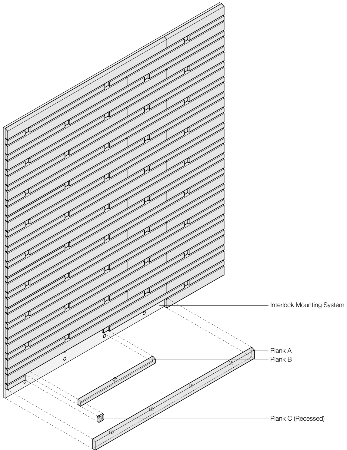
Exploded Axonometric
