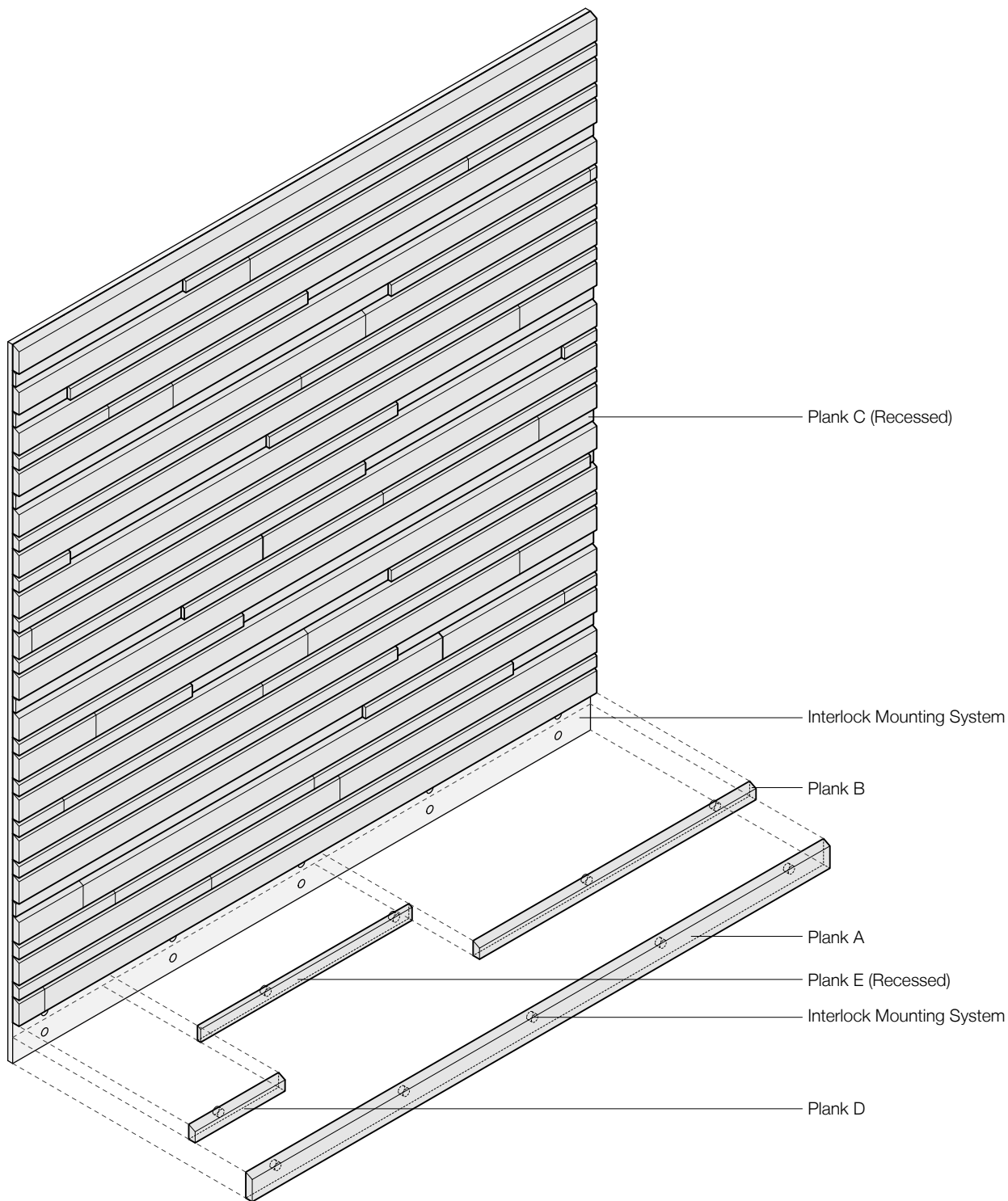
Exploded Axonometric
