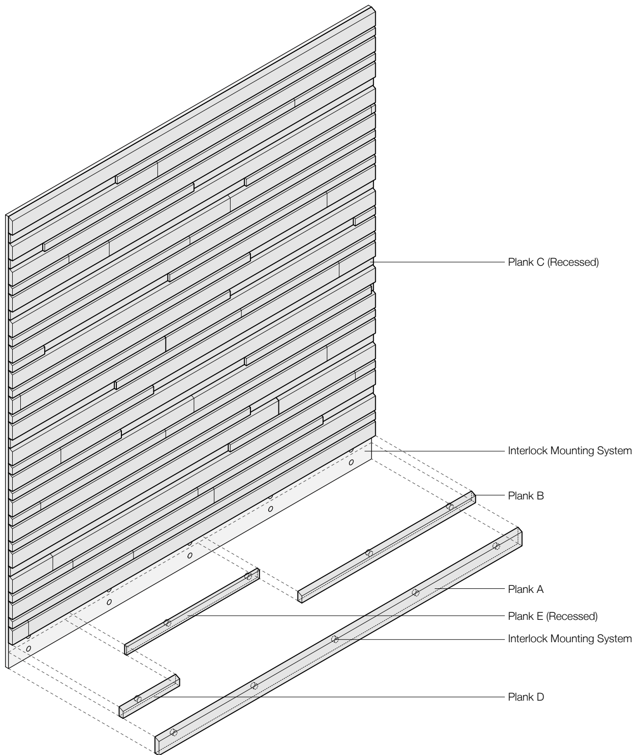
Exploded Axonometric
