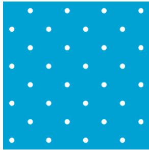
Pattern #330 .052 in. diameter diagonal 12 holes per square inch
