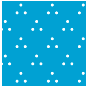
Multiple Diamond .052 in. diameter tri-star pattern 18 holes per square inch
