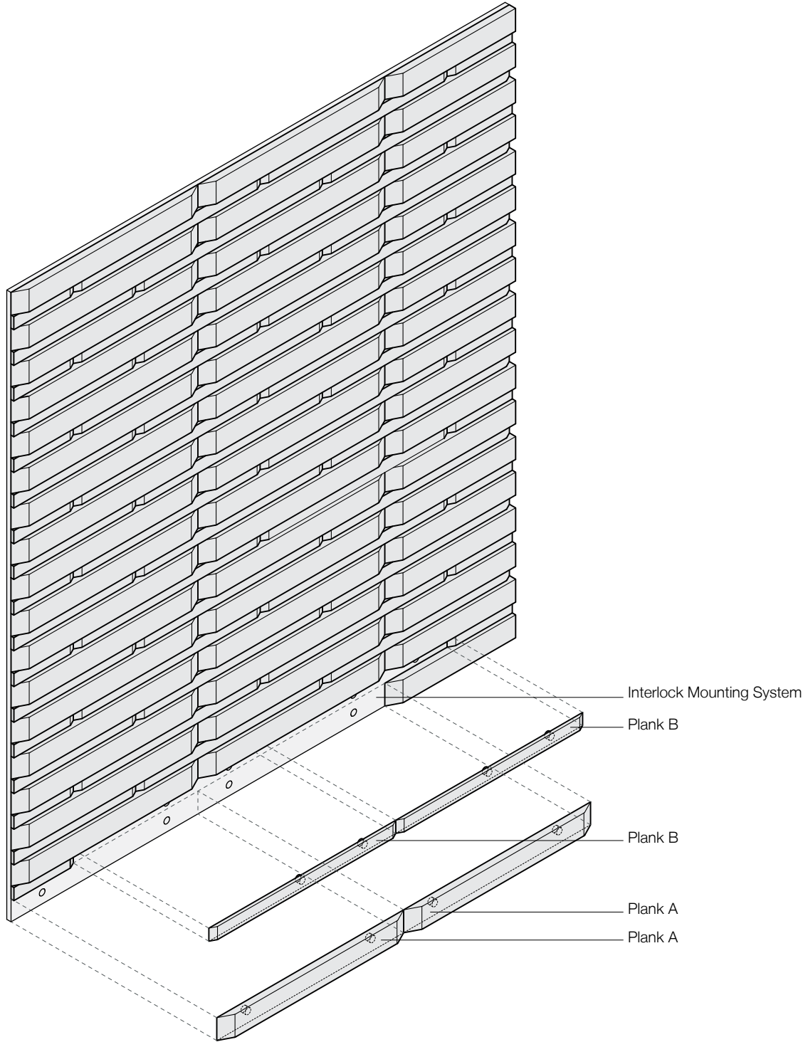
Exploded Axonometric
